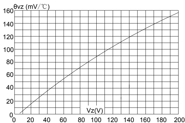
Fig.6 Temperature coefficient vs Zener voltage
